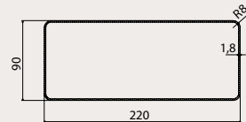
ROUND TO RECTANGULAR ADAPTER 220X90 MM cod. 112.0459.429
