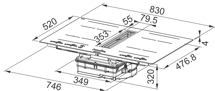
GALILEO CAN FIT IN 60/70 CM DEEP WORKTOP
