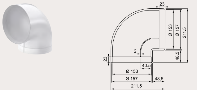
90° bend for round pipe 150
