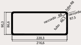
90° ELBOW BEND 220X90 MM cod. 112.0459.451
