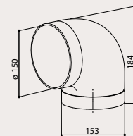
RIGHT ANGLE BEND 90° Ø 150 MM cod. 112.0253.688
