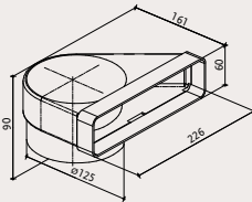
HORIZONTAL 90° BEND cod. 112.0157.300
