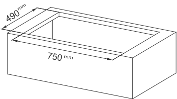
STANDARD INSTALLATION
