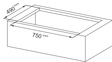
FLUSH FIT INSTALLATION
