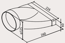
VERTICAL 90° ELBOW BEND cod. 112.0157.298
