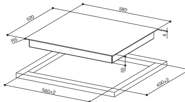
STANDARD INSTALLATION
