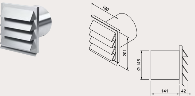
External outlet for round pipe with grid
