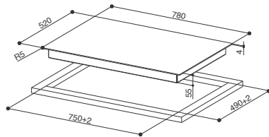
STANDARD INSTALLATION
