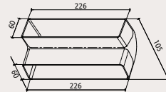
RECTANGULAR REDUCTION FITTING 60 MM cod. 112.0557.017
