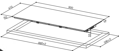
STANDARD INSTALLATION
