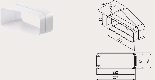
Horizontal 15° bend pipe
