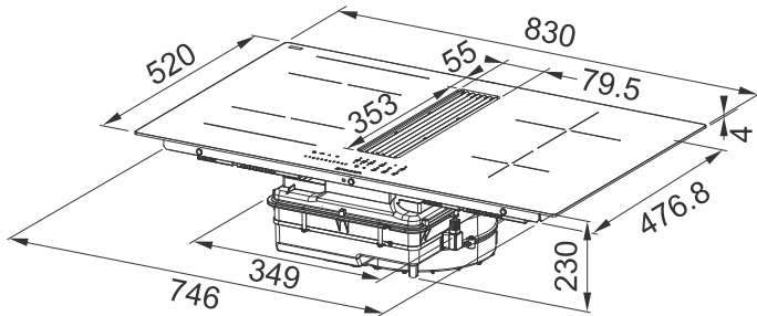
GALILEO CAN FIT IN 60/70 CM DEEP WORKTOP
