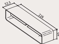
FLAT DUCT CONNECTOR cod. 112.0157.295
