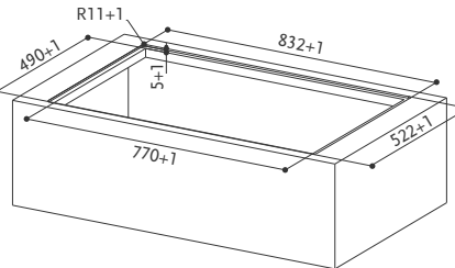
FLUSH FIT INSTALLATION
