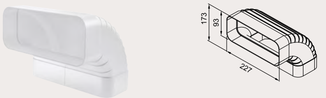
Pipe 150 vertical 90° bend
